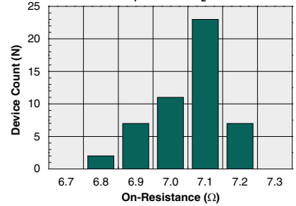
Typical On-Resistance Distribution (N=50, I_F=0.5mA , I_L=75mA )
