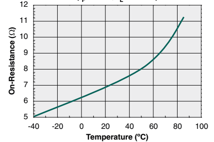
Typical On-Resistance vs. Temperature ( I_F=1mA , I_L=50mA )
