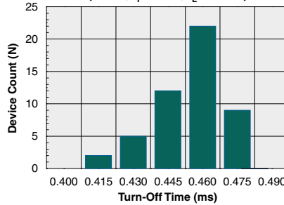
Typical Turn-Off Time (N=50, I_F=2mA , I_L=75mA )
