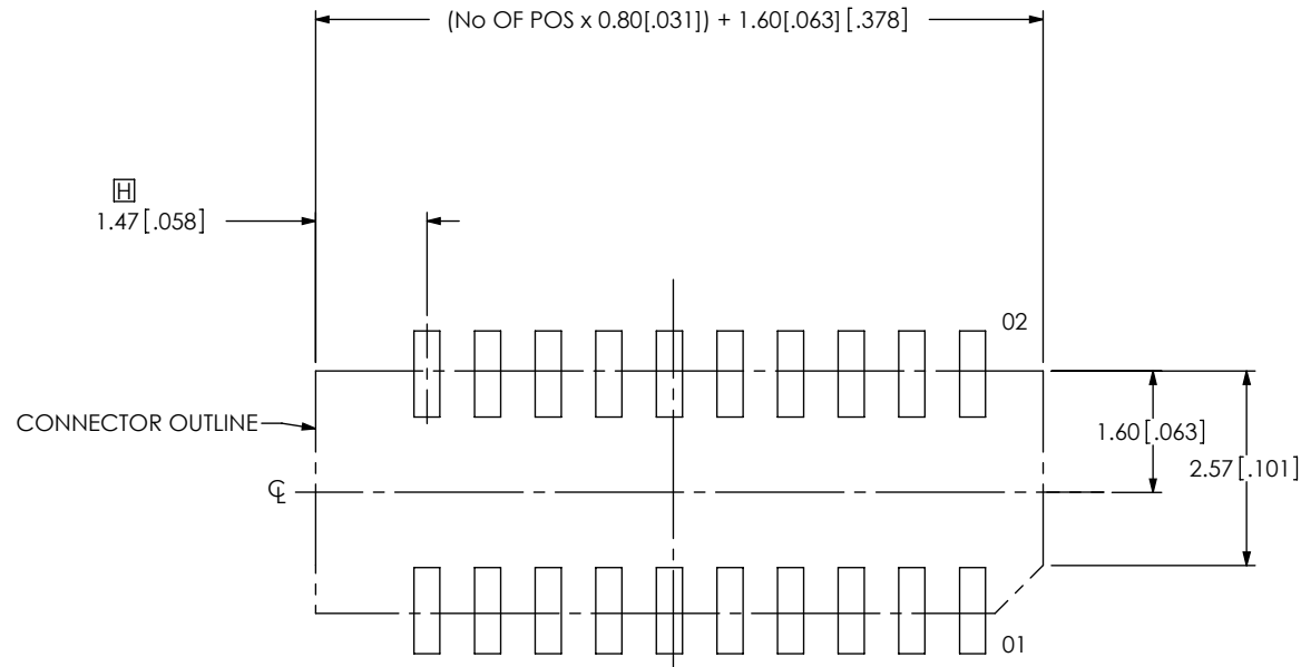
C CONNECTOR FIG 4 (SEMS-110-02-03.0-XX-D SHOWN) (SAME AS FIG 1, DIFFERENT AS SHOWN)
