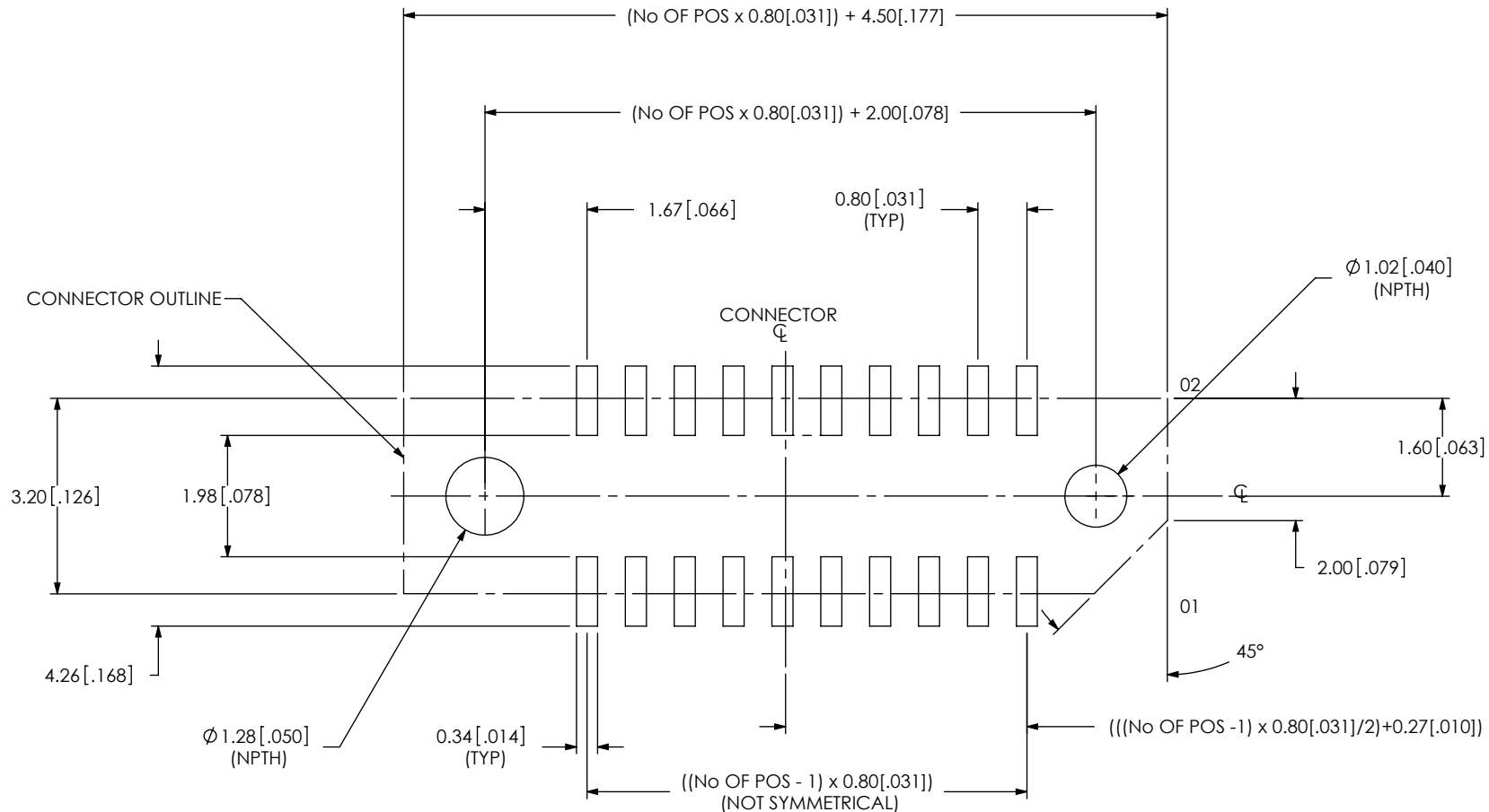
FIG 1 (SEM-110-02-03.0-XX-D-A SHOWN)
