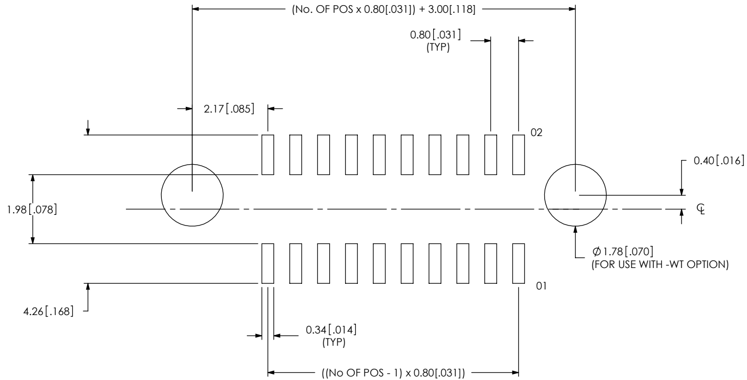
FIG 5 (SEMX-110-02-03.0-XX-D-WT SHOWN)
