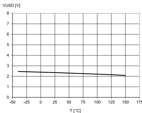
Figure 14: Undervoltage shutdown
