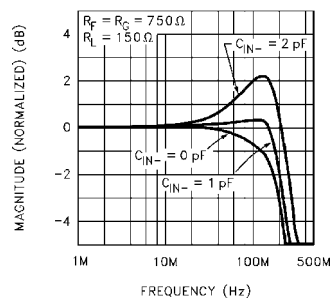
FREQUENCY RESPONSE FOR VARIOUS C_{IN-}
