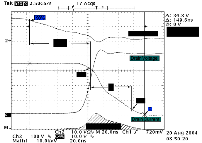
Figure 19, Turn-off Switching Waveforms and Definitions
