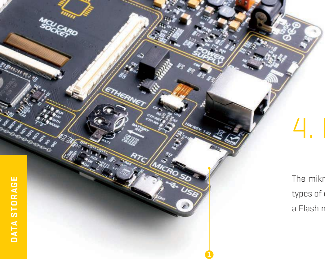
Figure 10: MicroSD card slot view
