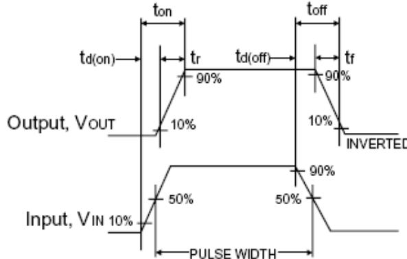
Switchin Waveforms
