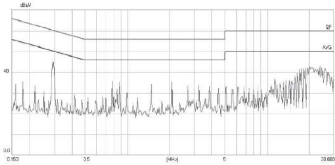
FILTER MODEL (VFM-10A) DC-DC CONVERTER MODEL: VHB50W-Q24-S5 Vin = 12 Vdc
