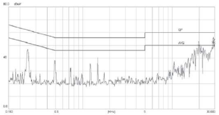
FILTER MODEL (VFM-25C) DC-DC CONVERTER MODEL: VHK200W-Q24-S12 Vin = 24 Vdc
