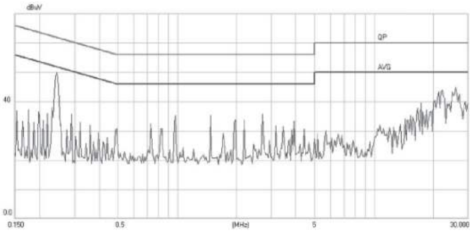
FILTER MODEL (VFM-20A) DC-DC CONVERTER MODEL: VHB150W-Q24-S5 Vin = 12 Vdc
