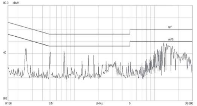
FILTER MODEL (VFM-25C) DC-DC CONVERTER MODEL: VHK200W-Q24-S12 Vin = 24 Vdc
