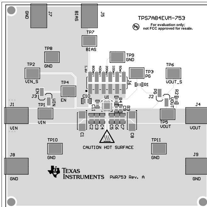
Figure 1. Assembly Layer
