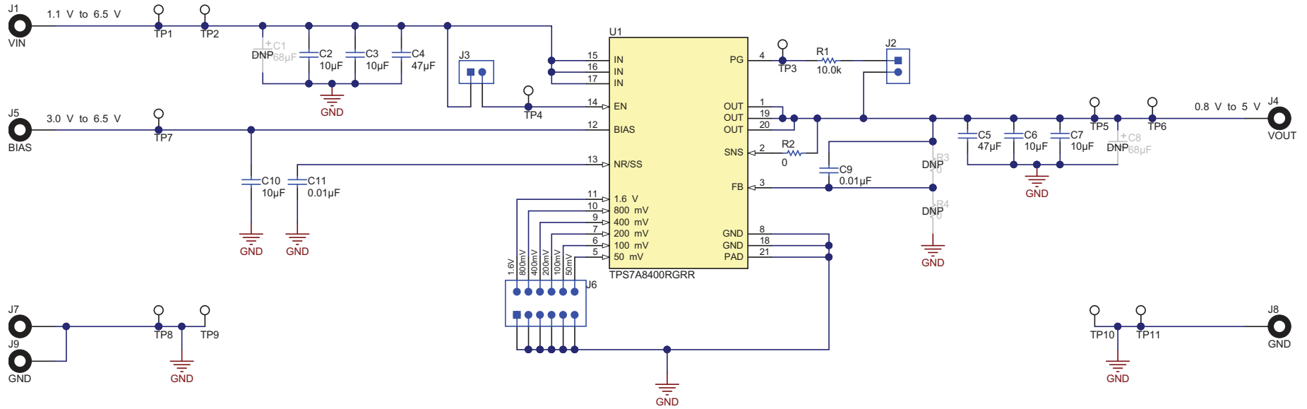
Figure 6. TPS7A84EVM-753 Schematic
