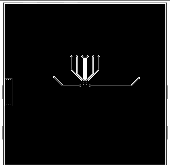
Figure 4. Signal Layer 2 Routing
