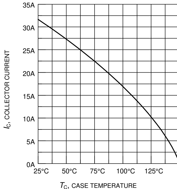
Figure 4. Collector current as a function of case temperature ( V_{GE} \leq 15\text{V} , T_i \leq 150^\circ\text{C} )
