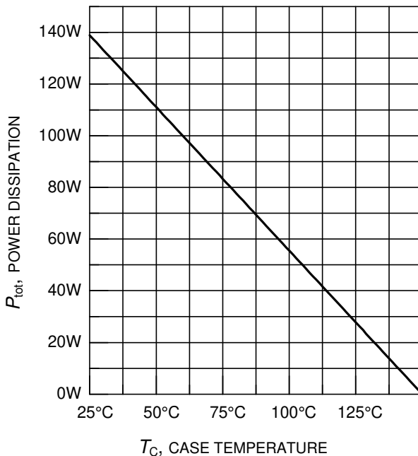
Figure 3. Power dissipation as a function of case temperature ( T_i \leq 150^\circ\text{C} )
