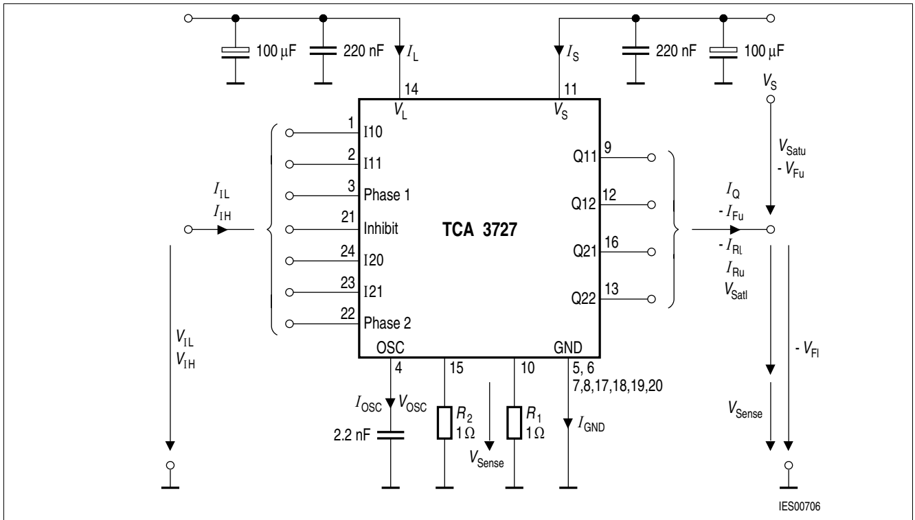
Figure 3 Test Circuit
