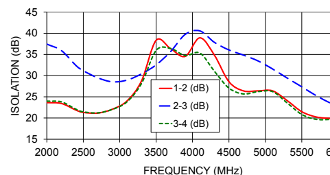
ZN4PD1-63-S+ ISOLATION
