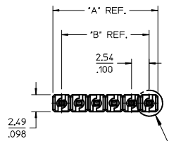
SEE DETAIL Z
