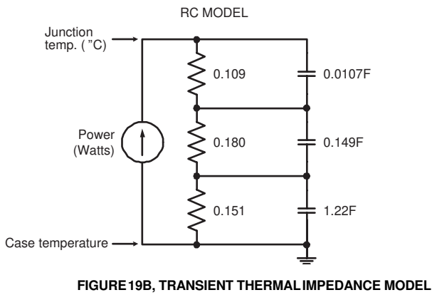
FIGURE 19B, TRANSIENT THERMAL IMPEDANCE MODEL
