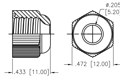
Ⓔ Sealing Nut
