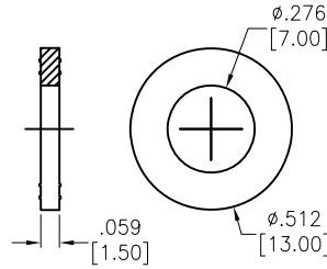
Ⓑ Washer
