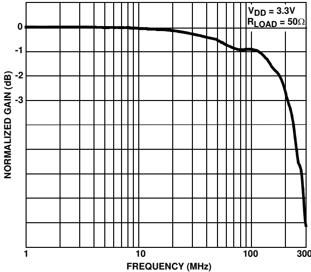
FIGURE 29. FREQUENCY RESPONSE
