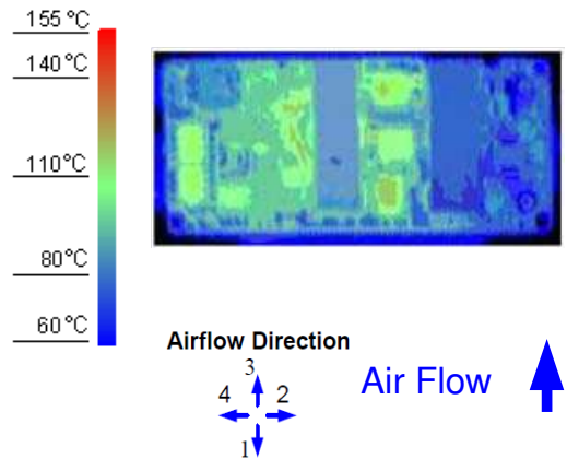
Figure 12. Thermal Image for Airflow Direction 3 (10A output, 55°C ambient, 200 LFM, typical V_{in} , open frame, socket interface)
