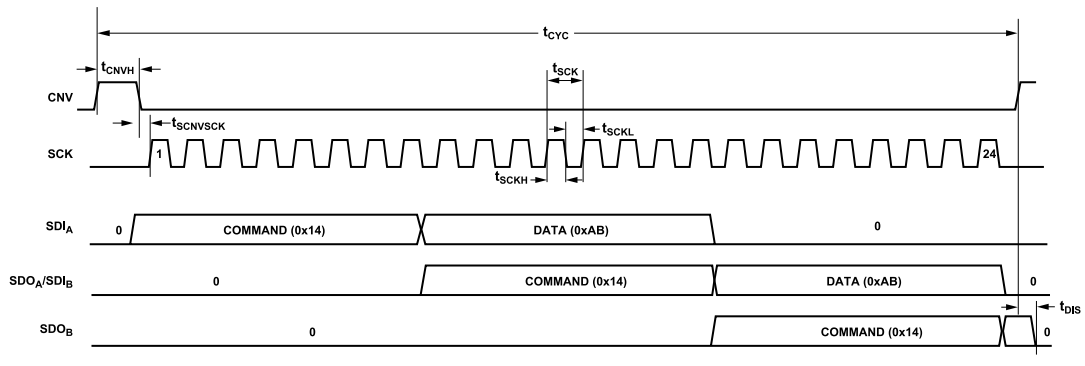
Figure 47. Register Write Timing Diagram, Daisy-Chain Mode
