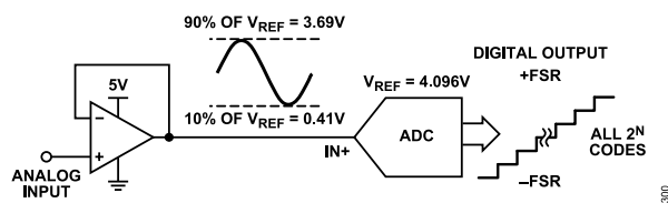
Figure 42. Span Compression
