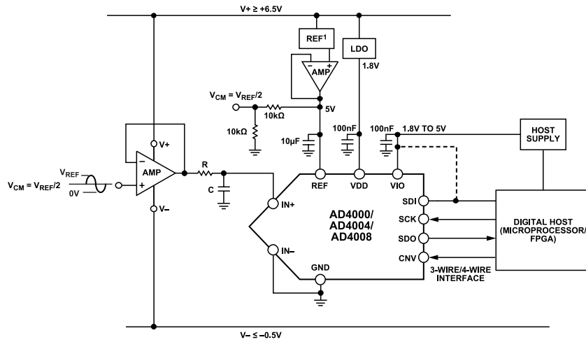
Figure 38. Typical Application Diagram with Multiple Supplies
