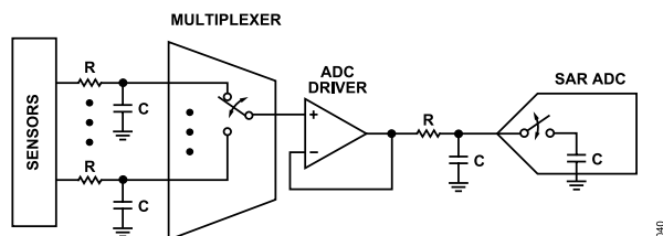
Figure 41. Multiplexed Data Acquisition Signal Chain Using the AD4000/AD4004/AD4008
