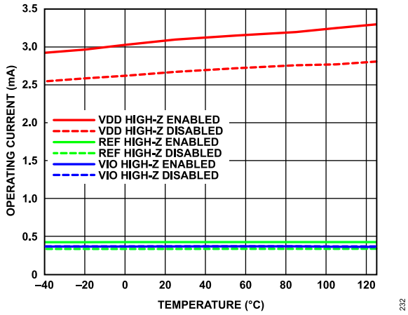
Figure 29. Operating Current vs. Temperature, AD4004, 1 MSPS
