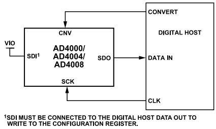
Figure 51. \overline{CS} Mode, 3-Wire Without Busy Indicator Connection Diagram
