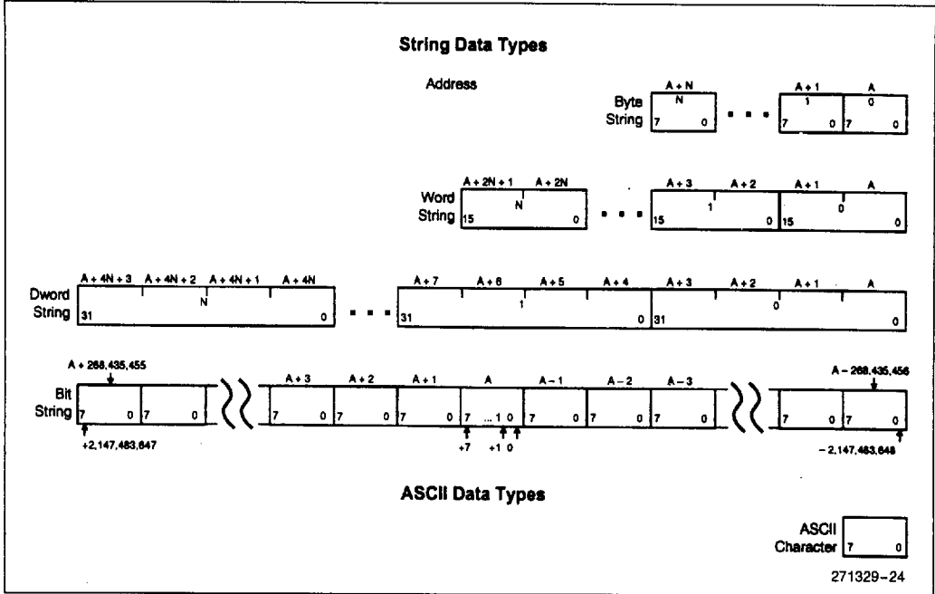
Figure 4-20. String and ASCII Data Types
