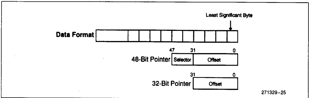
Figure 4-21. Pointer Data Types
