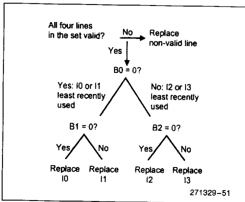
Figure 7-2. On-Chip Cache Replacement Strategy
