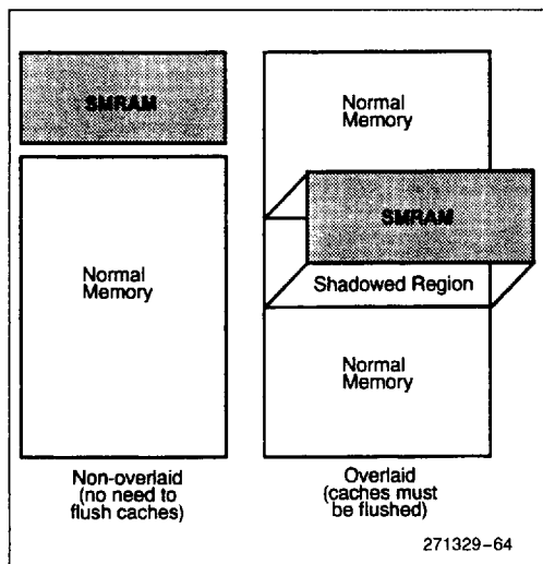
Figure 8-12. SMRAM Location
