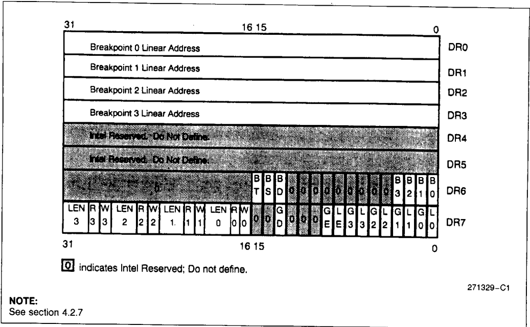
Figure 12-1. Debug Registers
