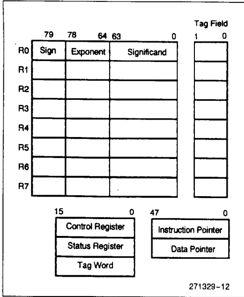
Figure 4-8. Floating Point Registers
