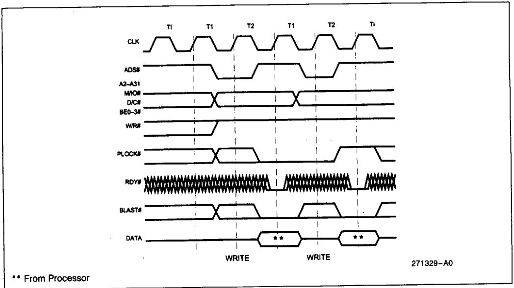
Figure 10-21. Pseudo Lock Timing
