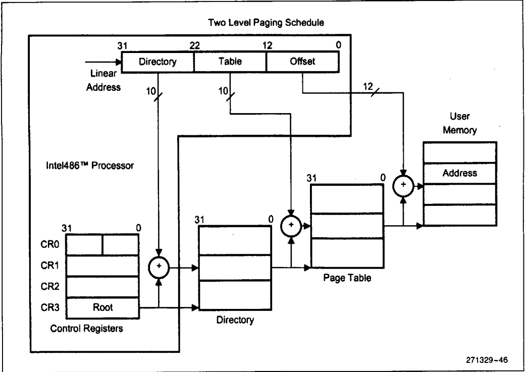
Figure 6-19. Paging Mechanism
