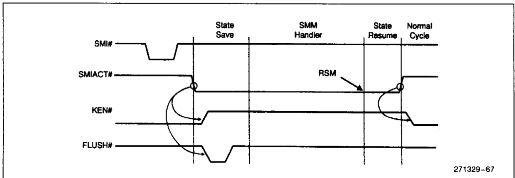
Figure 8-15. Non-Cached SMM
