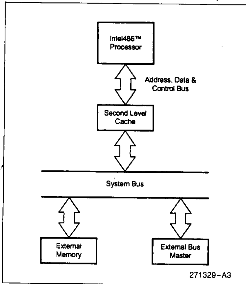
Figure 10-24. System with Second Level Cache
