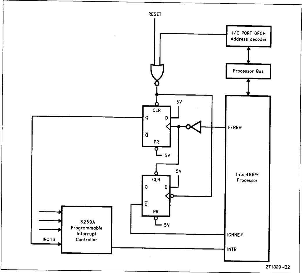
Figure 10-33. DOS-Compatible Numerics Error Circuit
