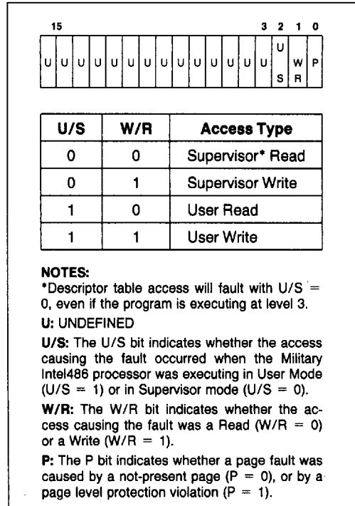
Figure 6-23. Page Fault System Information
