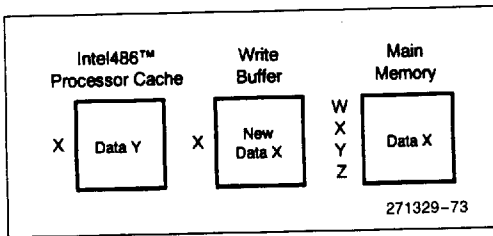
Figure 9-6. Reordering of a Reads with Write Buffers
