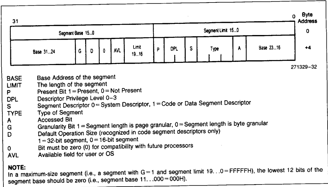
Figure 6-5. Segment Descriptors
