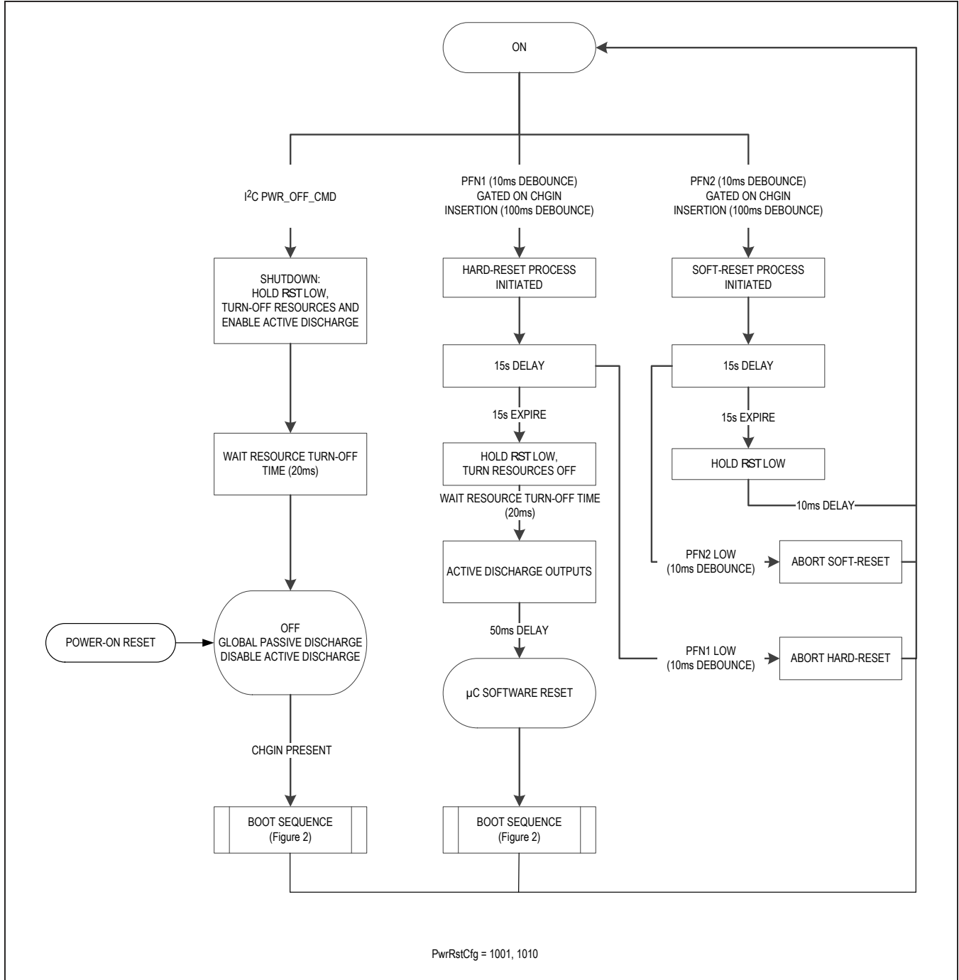
Figure 1g. PwrRstCfg = 1001, 1010
