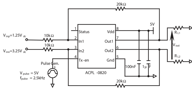
Figure 15. Tx enable/disable time test circuit.
