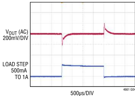
5V Output Load Transient Response
