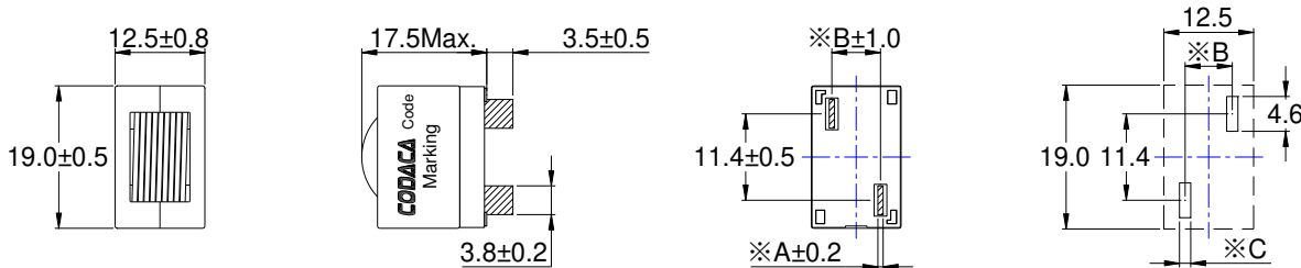
Typical Land pattern
