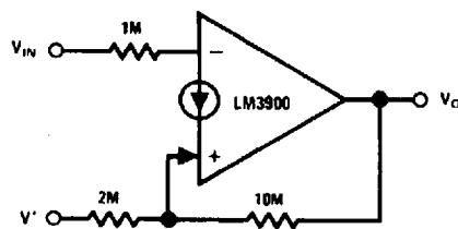
Schmitt-Trigger
