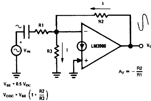
V_{BE} Biasing
