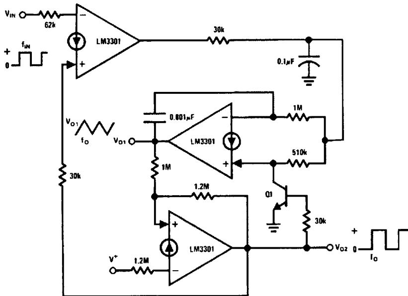
Phase-Locked Loop
