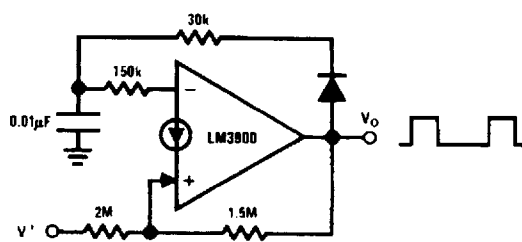
Pulse Generator
