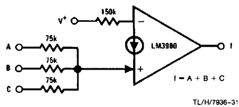
"OR" Gate
