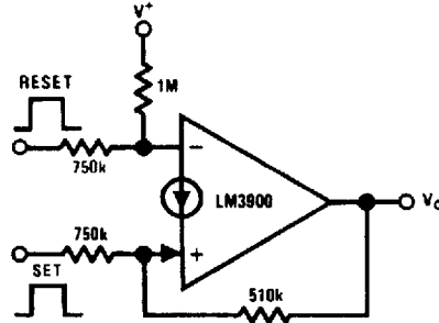
Bi-Stable Multivibrator
