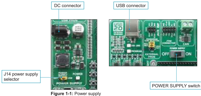
Figure 1-1: Power supply
