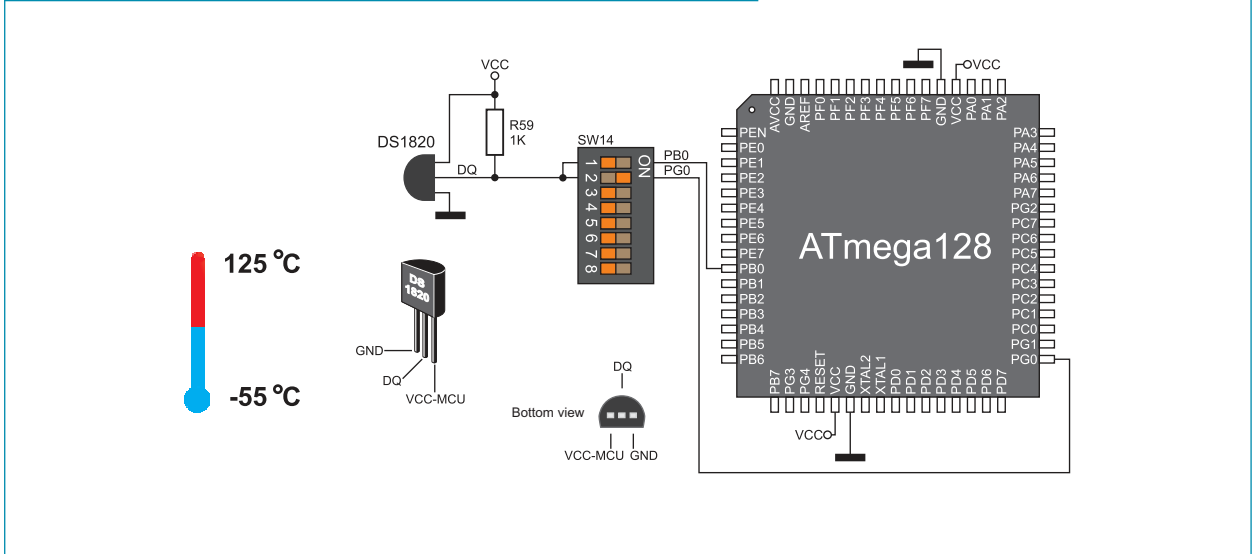
Figure 13-5: DS1820 and microcontroller connection schematic
