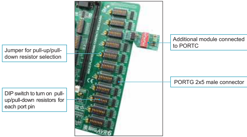
Figure 21-1: I/O ports
