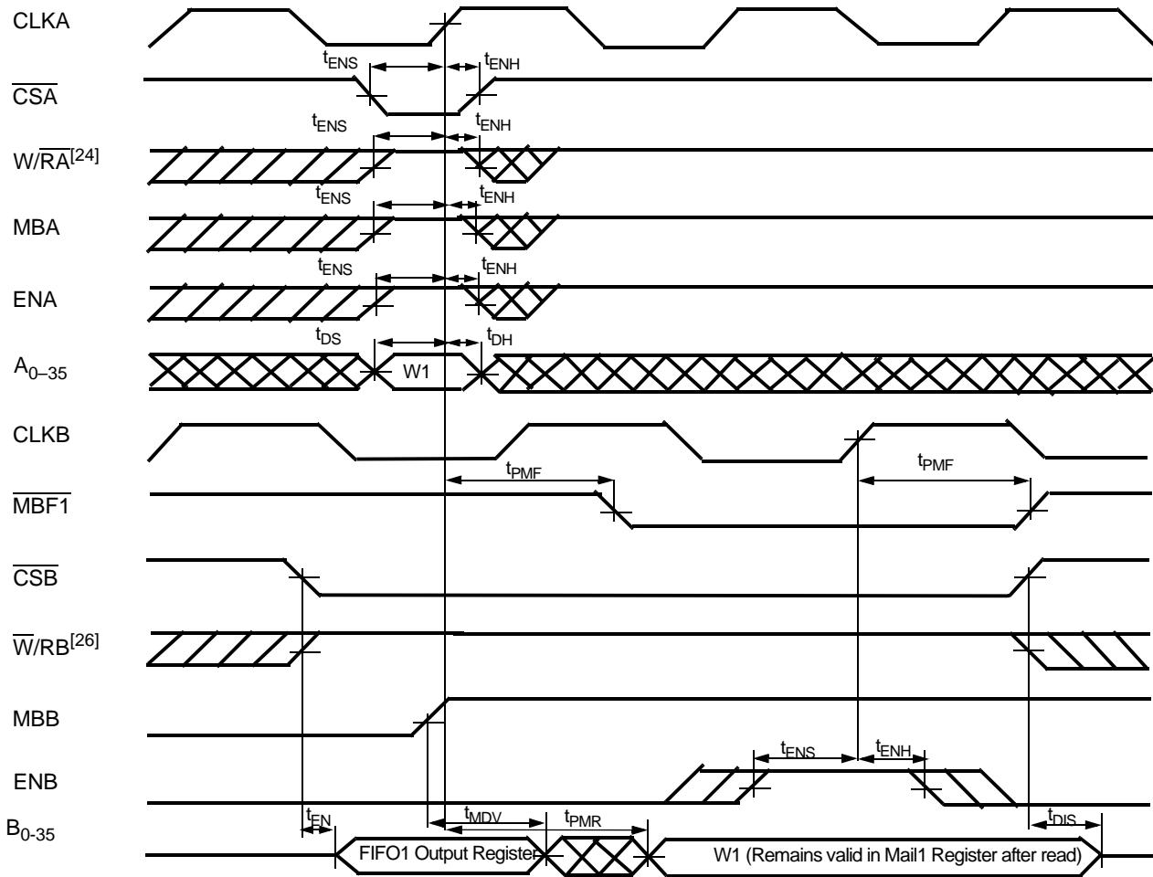
Timing for Mail1 Register and MBF1 Flag (CY Standard and FWFT Modes) [49]
