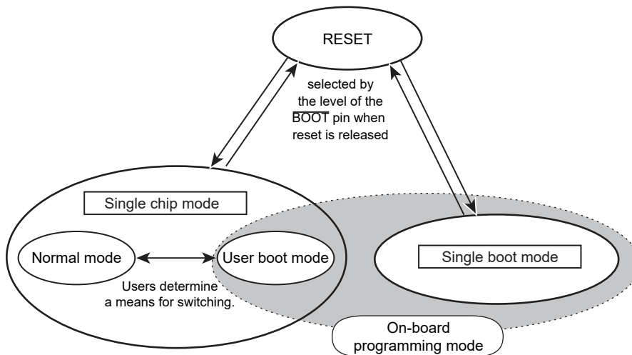
Figure 22-2 Mode transition
