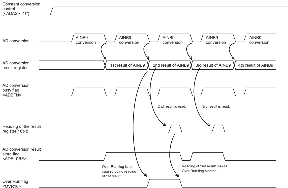
Figure 13-6 Constant conversion
