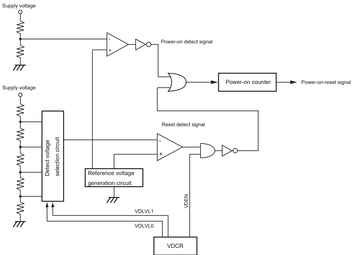
Figure 18-1 Power-on-reset circuit
