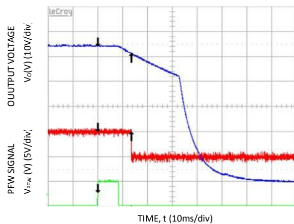
Figure 12. PFW alarmed 19.6ms prior to V o < 40V, output load: 38A, V IN = 185V AC .
