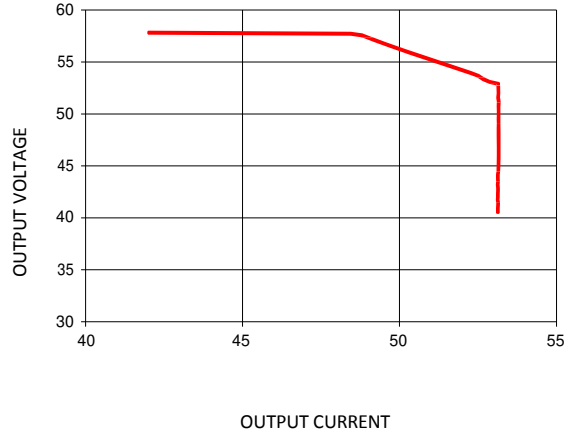
Figure 2. 54V DC output: Power limit, Current limit and shutdown profile at V IN = 185V AC .
