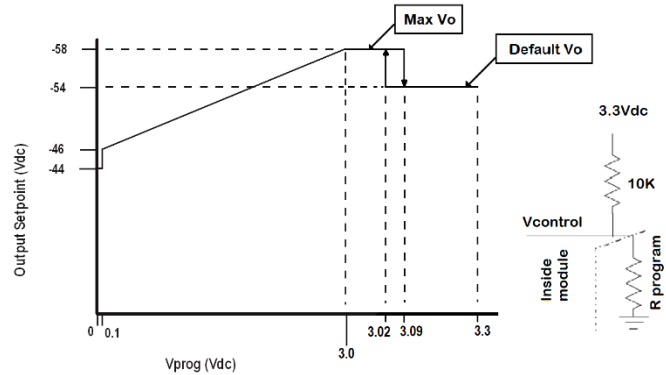
Figure 13. Diagram showing how output can be margined using Vcontrol adjustment.
