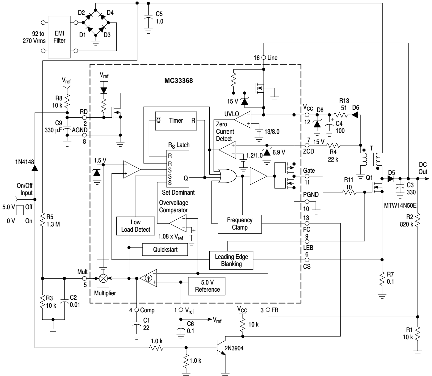
Figure 19. On/Off Control
