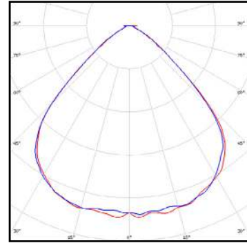
WWW - Very Wide High Bay Series
