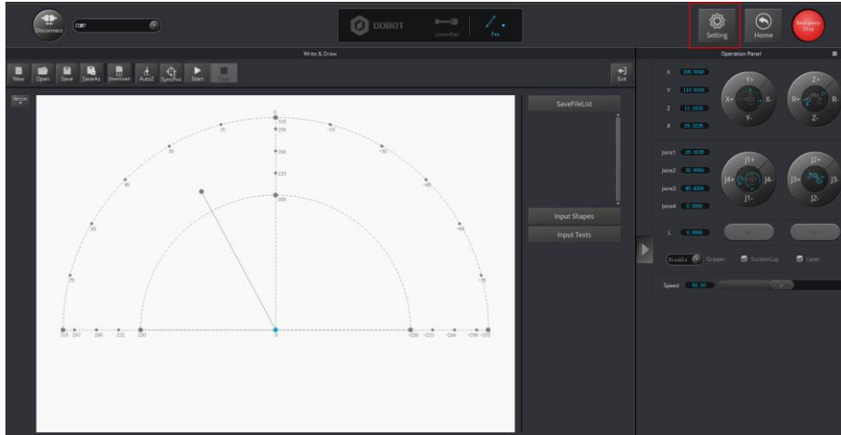
Figure 5.49 Click Setting
