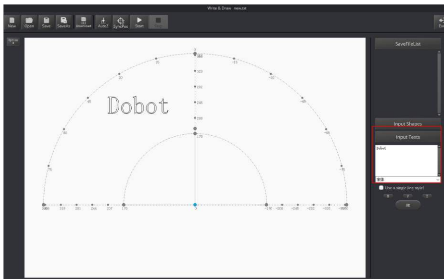
Figure 5.45 Input text
