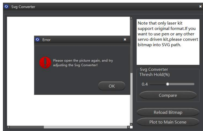
Figure 5.48 Error tip
