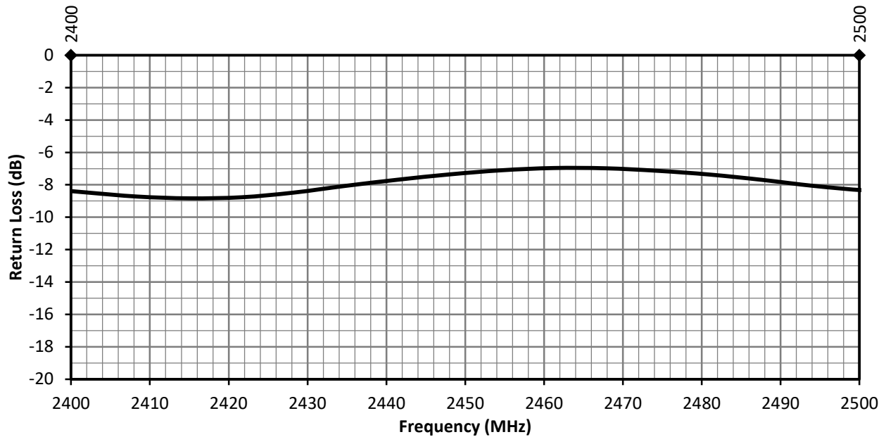
Figure 12. ANT-2.4-MMG2-SMA Antenna Return Loss, Free Space
