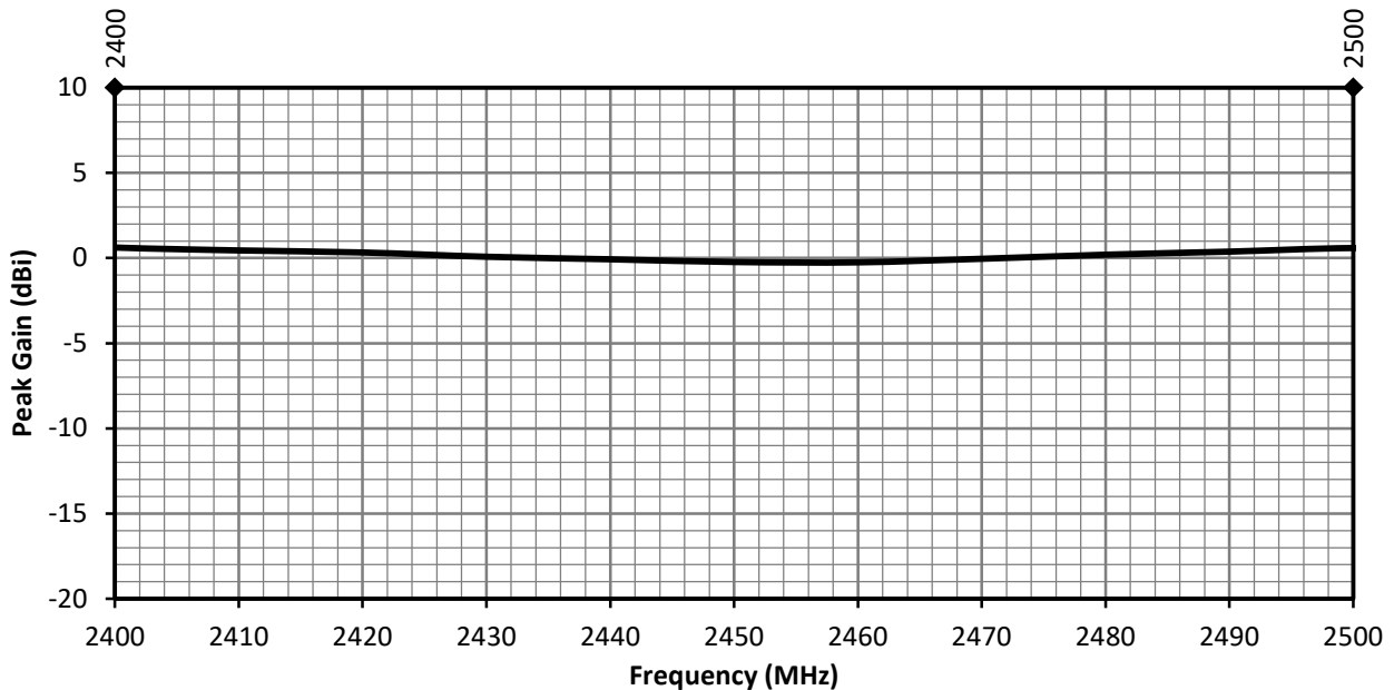
Figure 13. ANT-2.4-MMG2-SMA Antenna Peak Gain, Free Space
