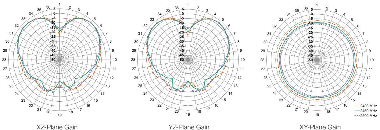
Figure 9. Radiation Patterns for ANT-2.4-MMG2-SMA Antenna on Ground Plane
