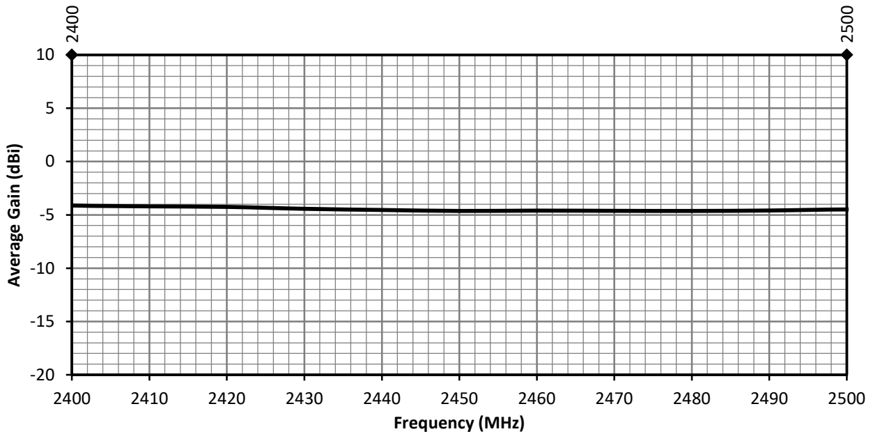
Figure 14. ANT-2.4-MMG2-SMA Antenna Average Gain, Free Space
