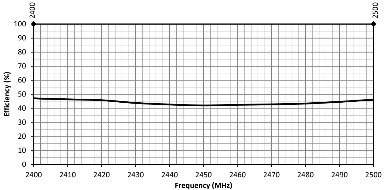
Figure 8. ANT-2.4-MMG2-SMA Antenna Radiation Efficiency on Ground Plane
