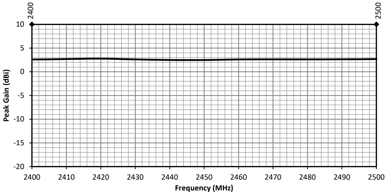
Figure 6. ANT-2.4-MMG2-SMA Antenna Peak Gain on Ground Plane
