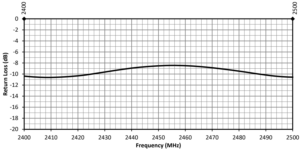
Figure 5. ANT-2.4-MMG2-SMA Antenna Return Loss on Ground Plane
