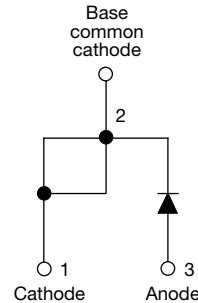
TO-247AC modified
