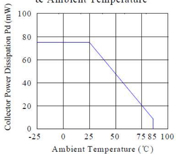
Collector Power Dissipation & Ambient Temperature
