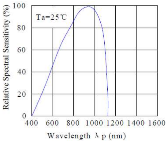
Spectral Sensitivity
