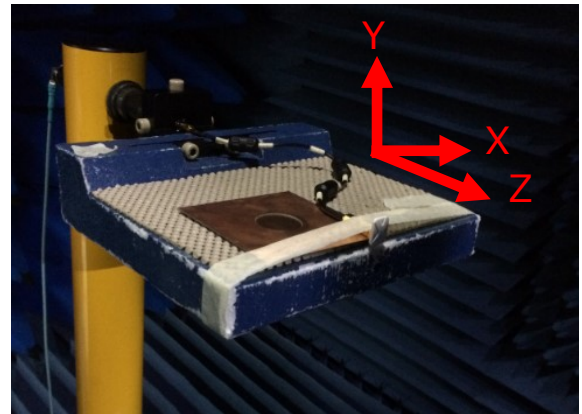
On 10*10cm ground plane (Off Center Edge)
