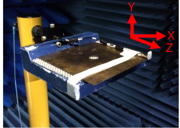
On 20*20cm ground plane (Off Center Edge)
