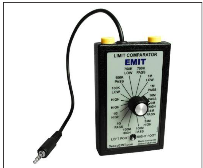
Figure 13. EMIT 50424 Limit Comparator
