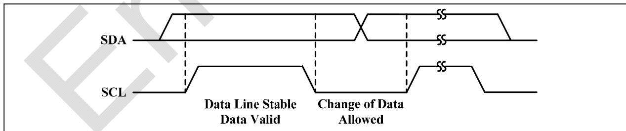
Figure 33 Bit Transfer
