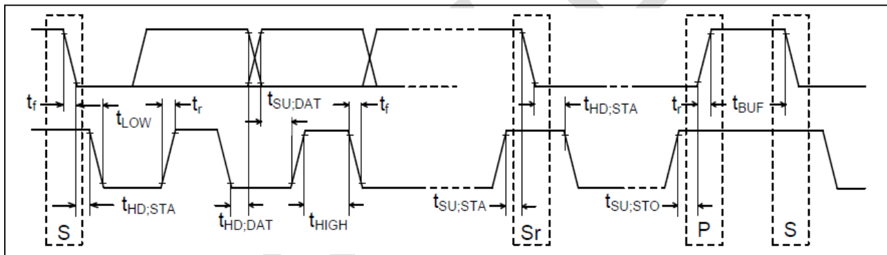
Figure 4 I2C Timing
