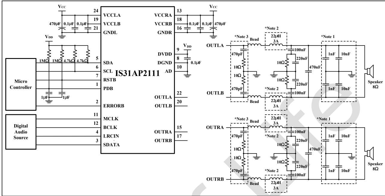
Figure 1 Typical Application Circuit (for BTL Stereo, Single-ended Input)
