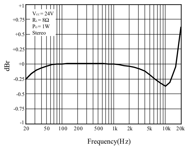
Figure 27 Frequency Response
