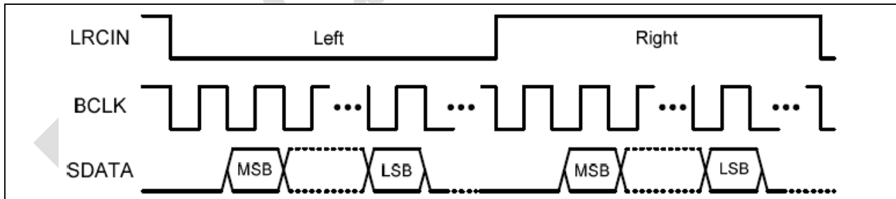
Figure 5 I2S
