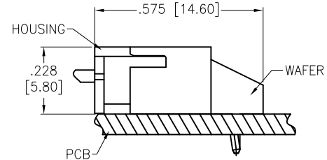
ASSEMBLY VIEW
