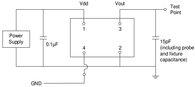
Figure 2. Test Circuit [10]
