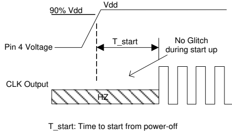
Figure 4. Startup Timing [11]
