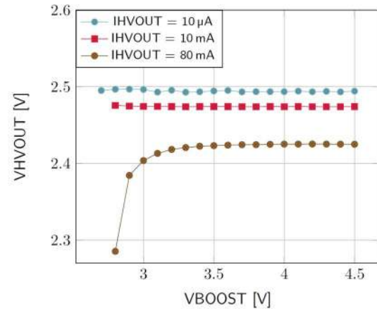
Figure 7: HVOUT at 2.5V
