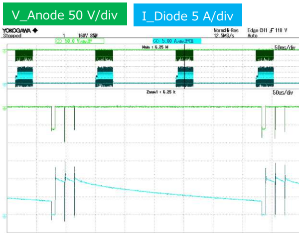
Figure 20. Output short V_{in\_dc} = 300\text{ V} Secondary side
