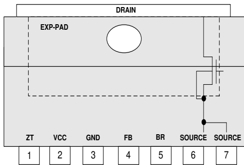
Figure 4. Pin Configuration
