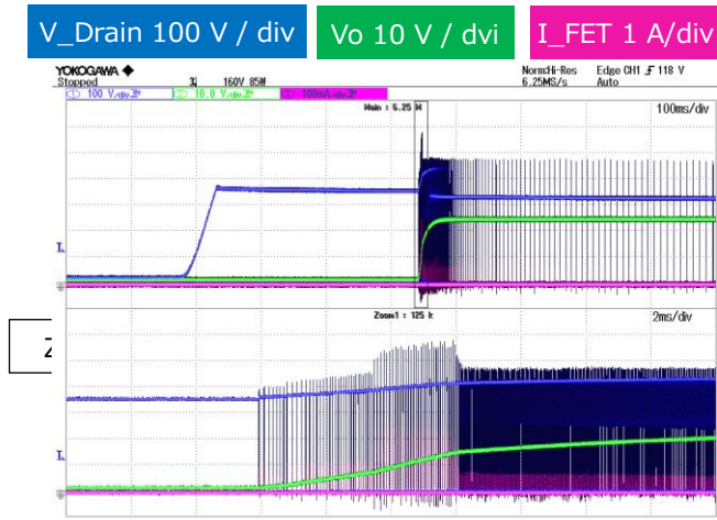
Figure 22. Startup V_{in\_dc} = 300\text{ V} , I_o = 0\text{ A}
