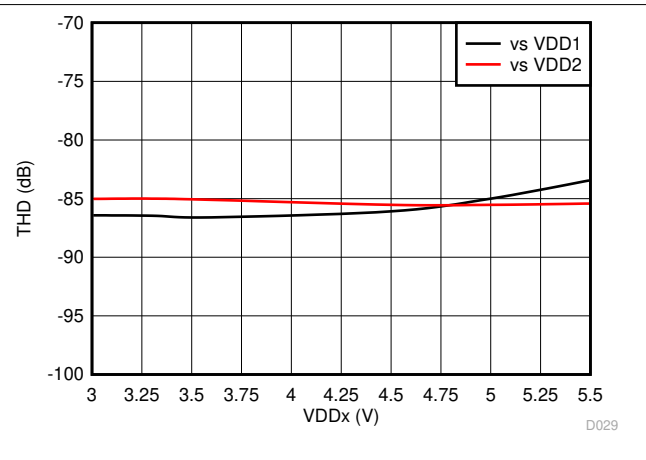
Figure 6-22. Total Harmonic Distortion vs Supply Voltage
