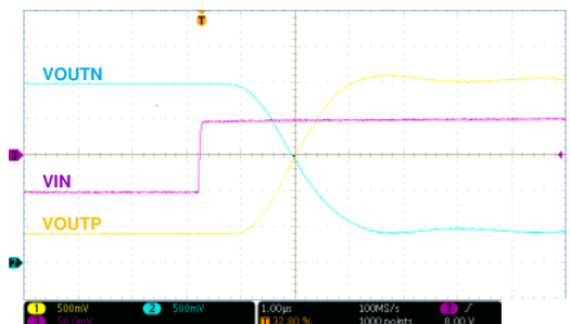
Figure 8-4. Step Response of the AMC1202
