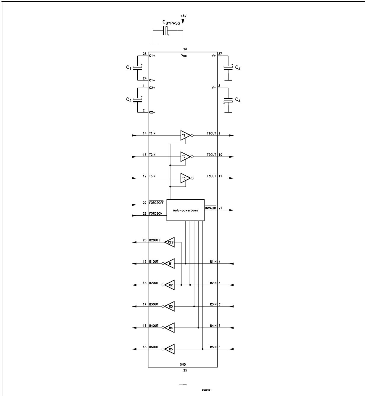
Figure 2. Application circuits
