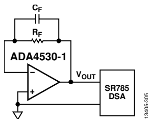
Figure 116. Current Noise Measurement Setup
