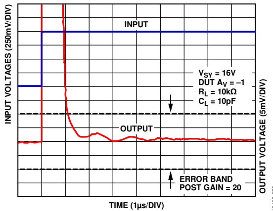
Figure 78. Positive Settling Time to 0.1%, V_{SY} = 16V
