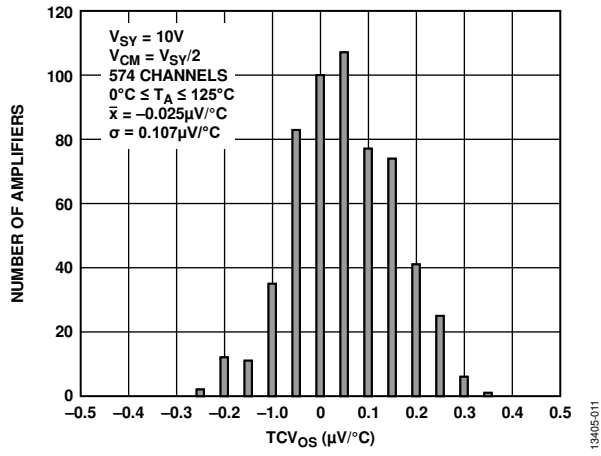
Figure 14. Input Offset Voltage Drift Distribution, 0^{\circ}\text{C} \leq T_A \leq 125^{\circ}\text{C} , V_{SY} = 10\text{ V}
