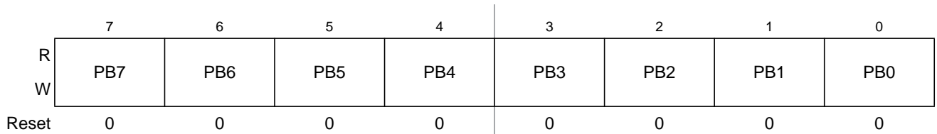
Figure 23-4. Port B Data Register (PORTB)
