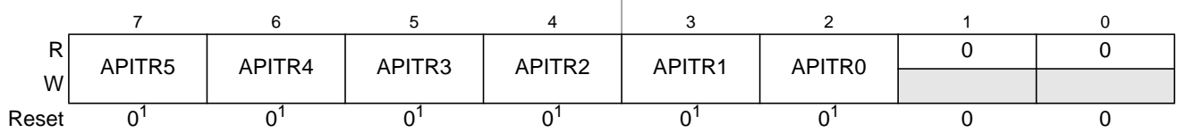
Figure 14-5. Autonomous Periodical Interrupt Trimming Register (VREGAPITR)
