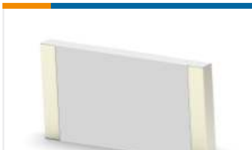
TE Part #7-2176246-6 CRGS2512 5% 1M8
