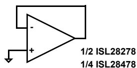
FIGURE 40. PREVENTING OSCILLATIONS IN UNUSED CHANNELS
