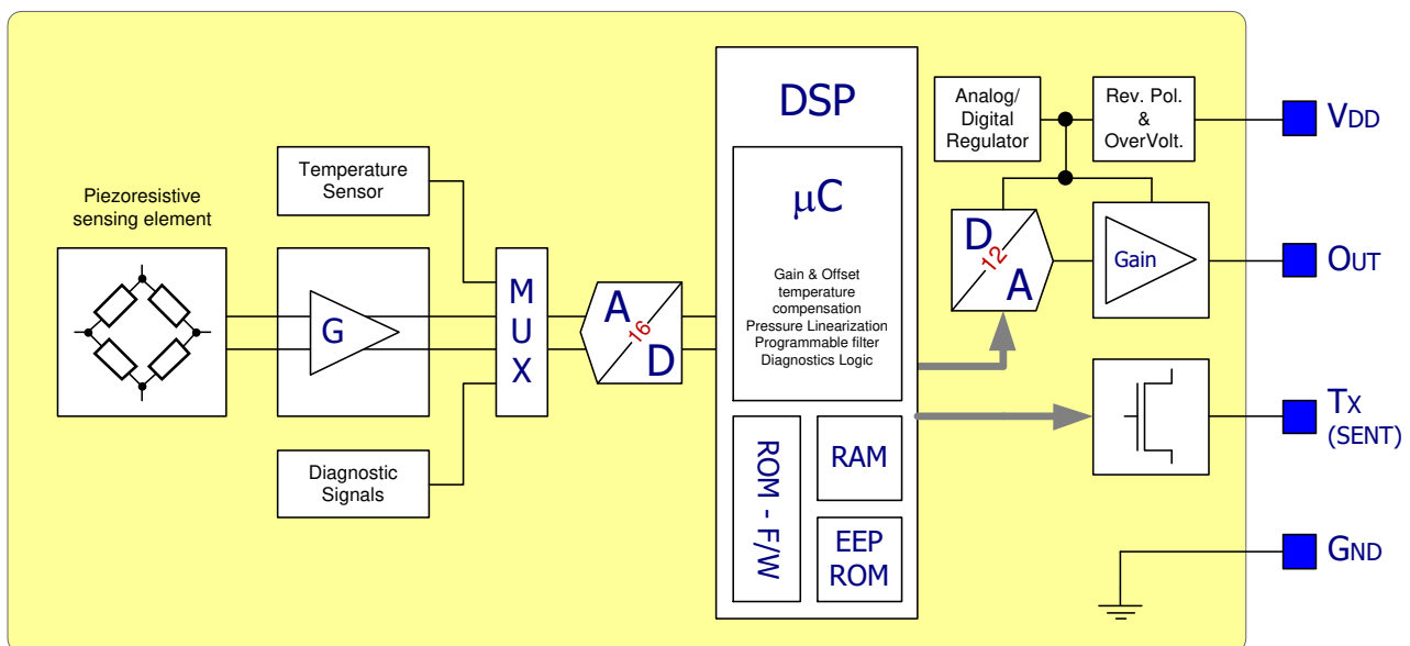
Figure 2: MLX90819 block diagram
