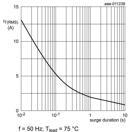
Fig. 2. RMS on-state current as a function of surge duration; maximum values f = 50\text{ Hz} ; T_{lead} = 75\text{ }^{\circ}\text{C}
