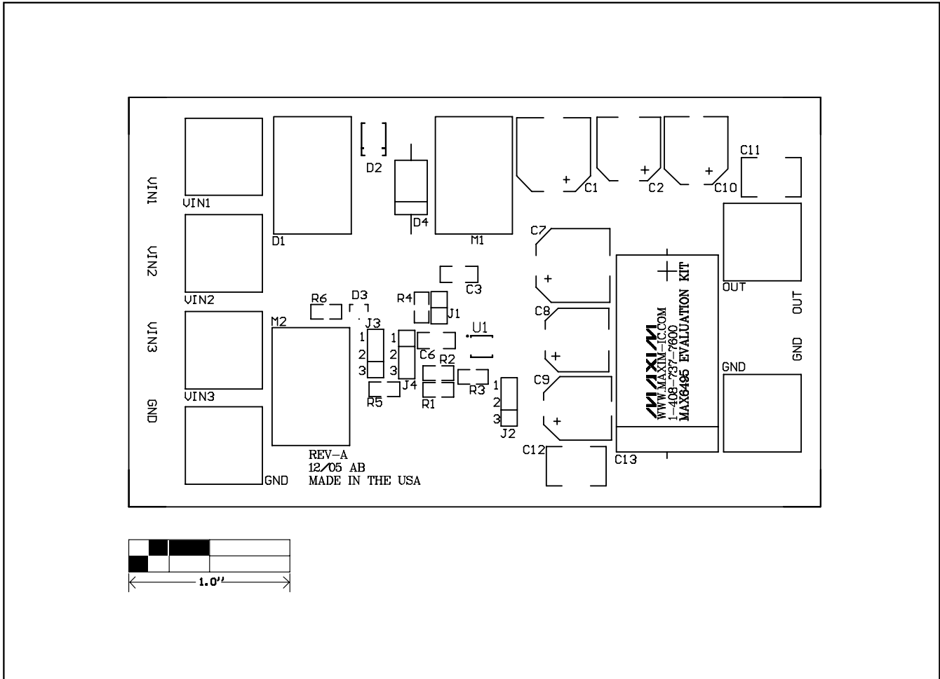
Figure 2. MAX6495 EV Kit Component Placement Guide—Component Side
